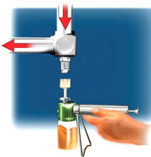
Figure 4. Drain line Vacuum Sampling
